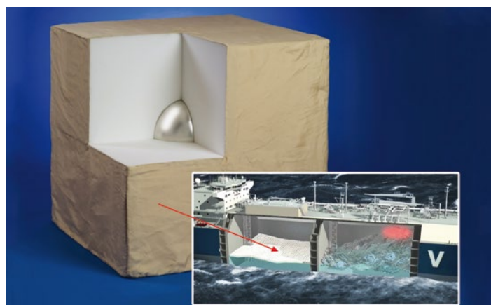
Basotect® cube for anti-sloshing. Photo: BASF/Samsung Heavy Industries
